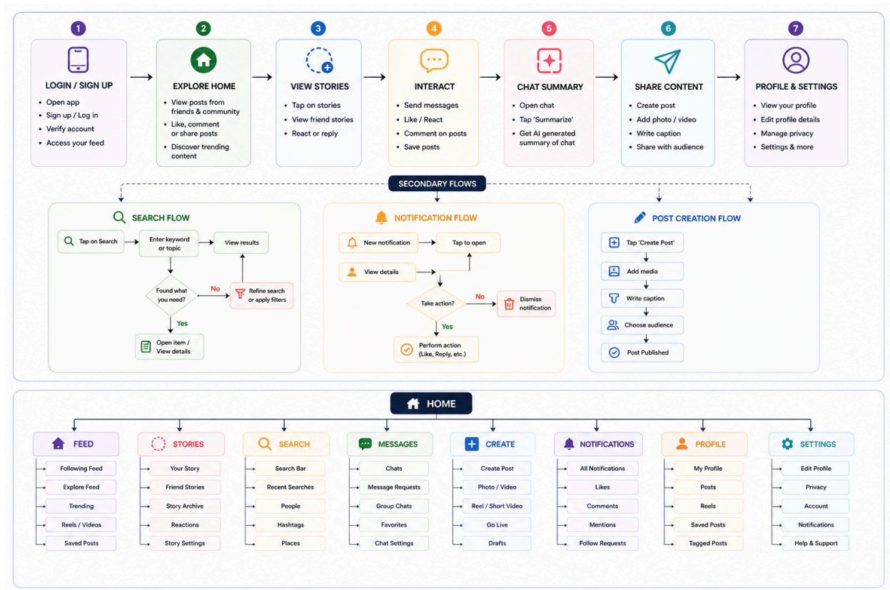
Fig. 6.1 Task Flow Diagram
