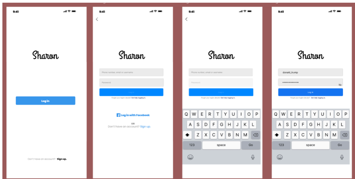
Fig. 7.1 User login and verification
